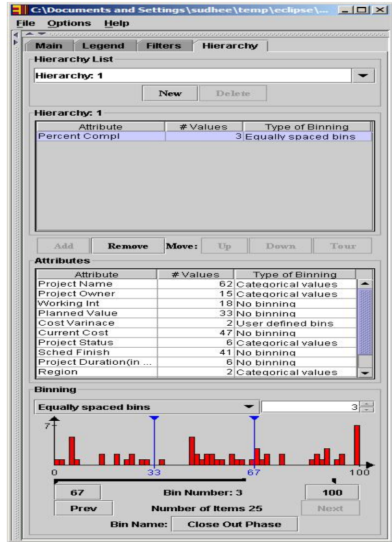
Figure 9: Revised Flexible Hierarchy user interface showing the binning widget at the bottom.
