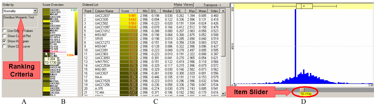
Figure 2. Rank-by-feature framework interface for histograms (1D) All 1D histograms are ordered according to the current order criterion (A) in the ordered list (C). The score overview (B) shows an overview of scores of all histograms. Mouseover event activates a cell in the score overview, highlights the corresponding item in the ordered list (C) and shows the corresponding histogram in the histogram browser (D) simultaneously. A double click on a cell enlarges the cell and activates it until another double click event occurs. A selected histogram is shown in the histogram browser (D), where users can easily traverse histogram space by changing the dimension for the histogram using item slider. Boxplot is also shown above the histogram to show the graphical summary of the distribution of the dimension. (A gene expression data set for melanoma study (3614 genes x 38 samples)).
