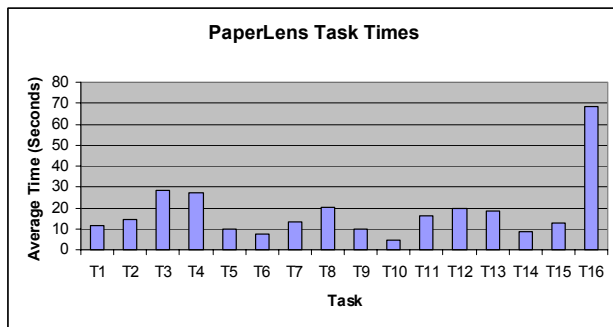
Figure 8. Average task times using PaperLens with the InfoVis proceedings.
