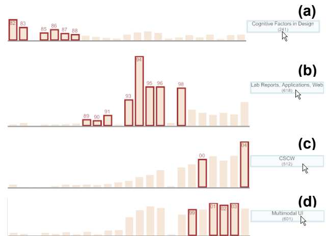
Figure 3. Highlighting of the most common topics: (a) Cognitive Factors in Design (b) Lab Reports, Application, Web (c) CSCW (d) Multimodal UI.
