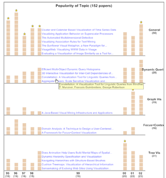
Figure 10. For the earlier prototype, a fisheye technique is used to help people reveal the individual paper titles for that year by topic when the user clicked on a year.
