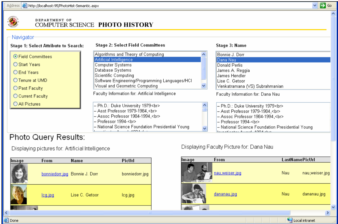
Figure 2: This figure shows the three stage process for querying the CS PhotoHistory libraries. The user chooses the initial attribute to query, then the browser fine-grains the search to all entities lying within that domain. Upon the second user selection, the browser retrieves a third-level list of results. Below the 'Navigator' are the actual photo results of the query listed alphabetically by last name.
