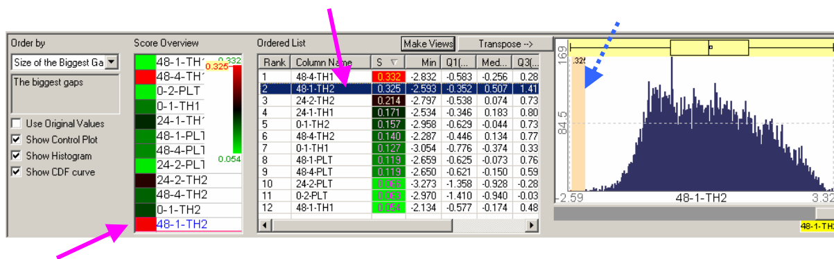
Figure 1 The biggest gap ranking result led P1 to make interesting discoveries. In this case the second biggest gap was especially interesting. It occurs in the histogram for 48-1-TH2 (purple arrow), and is shown as a peach color region (blue dotted arrow) on the left side of the histogram.
