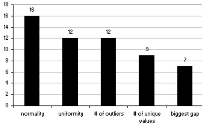
Figure 7 What are the most useful ranking criteria in the histogram ordering?
