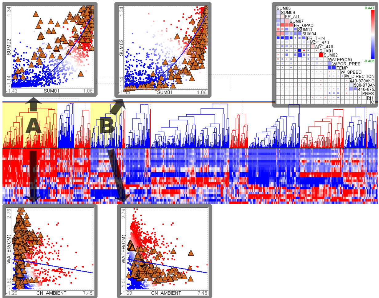
Figure 6 Ranking by quadracity in the aerosol data set and a dendrogram interaction. Score overview is at top right corner. The size of each cell represents 1 - (\text{least square error of regression}) , and the color of each cell represents the ranking score, or quadracity. The big bright red square at the center of the score overview represents the quadracity between SUM01 and SUM02, and the corresponding scatterplot is shown at the top. Clicking on the cluster A at the dendrogram, P3 can see that the items in the cluster (highlighted as brownish triangles) deviate from the regression curve as shown at the top left scatterplot, while the items in the cluster B are well-aligned with the curve at the top right scatterplot. The two scatterplots at the bottom show distinctive distributions of the two clusters (A and B) on another scatterplot (CN_AMBIENT vs. WATER).
