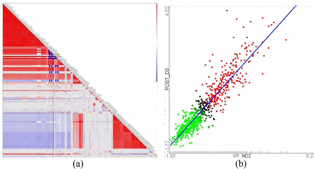
Figure 5 An improved score overview (a) and fitting result (b) with missing values excluded
