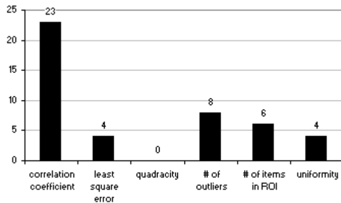
Figure 8 What are the most useful ranking criteria in the scatterplot ordering?
