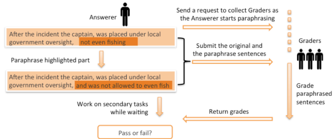
figure 1: FluTCHA workflow. The answerer on the left is the entity being tested for being human. The graders on the right help determine whether the entity on the left is human.
