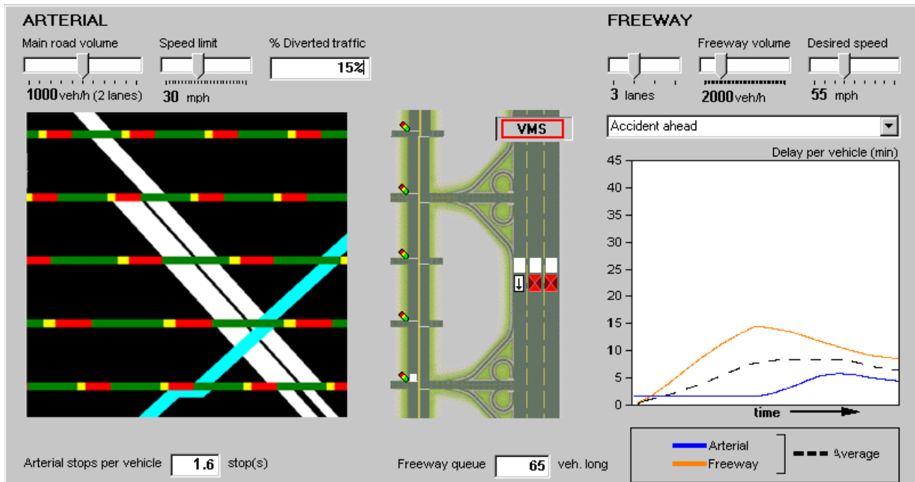
Figure 4: The signal timing of the 3 rd and 4 th intersections from the top was adjusted. Fewer vehicles have to wait for a second cycle at the 3 rd intersection. The arterial delays are reduced and the overall average delay as well. As users adjust the signal timing interactively on the time-space diagram, the effect on the bands is shown immediately and users can quickly explore alternatives. Users can then start checking the effect of the changes on the reverse direction traffic.
