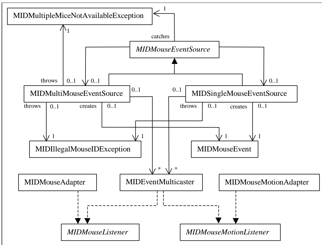
Figure 3: Class structure of MID in UML. Solid lines with solid arrows represent inheritance. Dashed lines with solid arrows represent implementation. Solid lines with open arrows represent associations. The numbers and text next to an association line represent cardinality and role of a class in the association.
