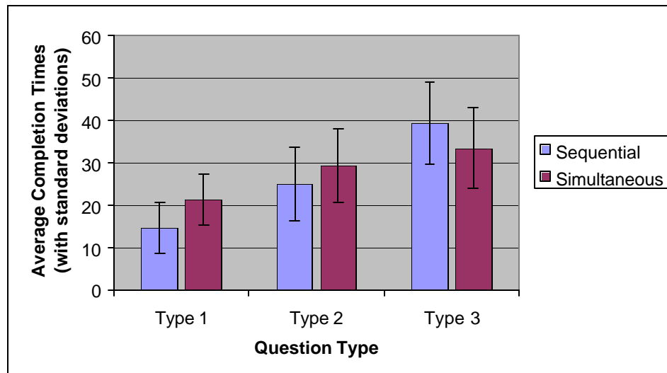
Figure 3: Experimental Results: Sequential menus produced better performance for Types 1 and 2, but simultaneous menus were faster for Type 3 ( n=20 ). Error bars indicate a range of one standard deviation from the mean.
