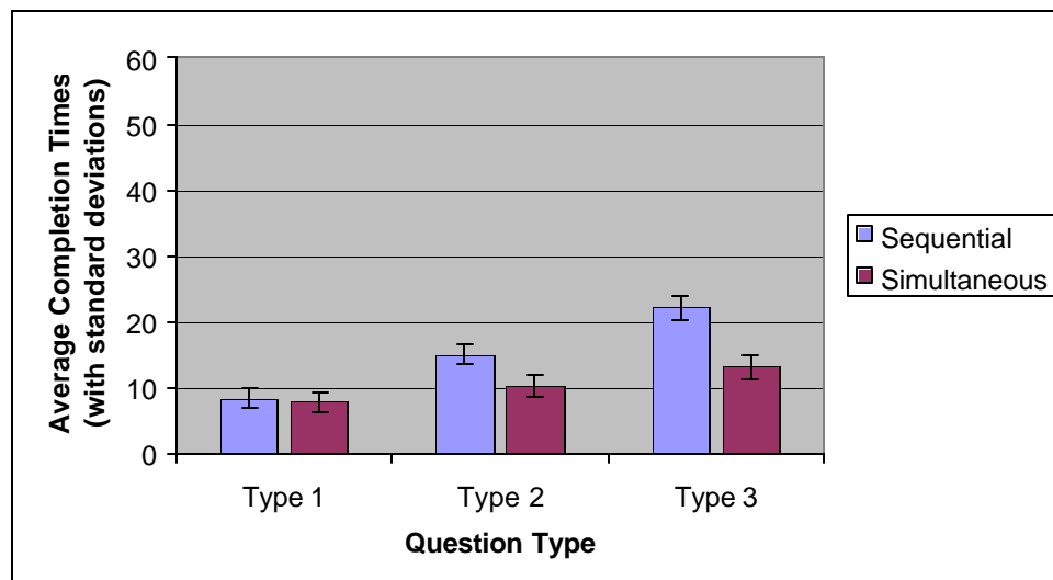
Figure 4: Estimated performance results for proficient users, based on composite results from three experienced users: Simultaneous menus are faster for all three types of questions, indicating a possible learning effect that may favor simultaneous menus.
