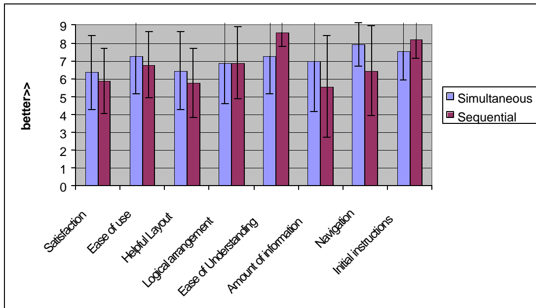
Figure 5: Subjective Questionnaire Results: Average values are shown for 20 subjects, with error bars indicating one standard deviation difference. Higher numbers are better results. Roughly comparable subjective responses to the two menu types provide some indication that users are not necessarily confused or disoriented by simultaneous menus.
